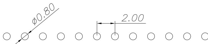
PCB. LAYOUT
