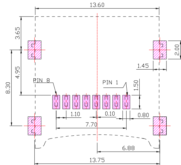
PCB LAYOYT
