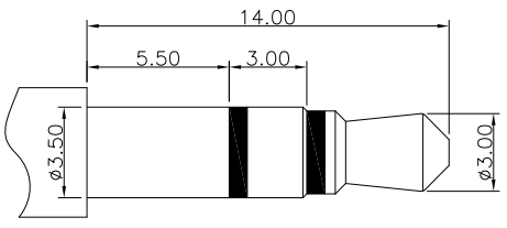
3.50mm 3 POLE PLUG
