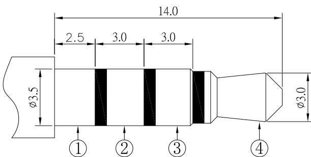
φ3.50mm 4 POLE PLUG
