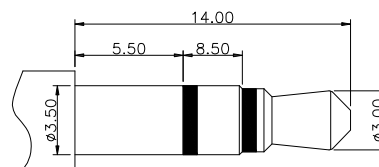
φ3.50mm 3 POLE PLUG
