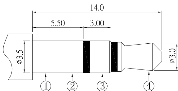
Ø3.50mm 3 POLE PLUG
