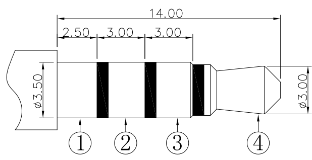
Ø3.50mm 4 POLE PLUG
