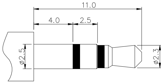
∅2.50mm 3 POLE PLUG
