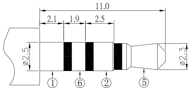
\phi 2.50mm 4 POLE PLUG
