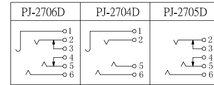
SCHEMATIC
