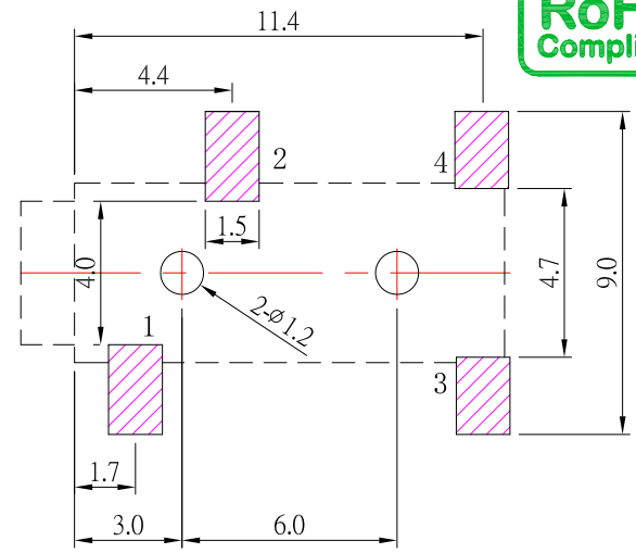
P.C.B LAYOUT MOUNTING PATTERN (TOP VIEW)
