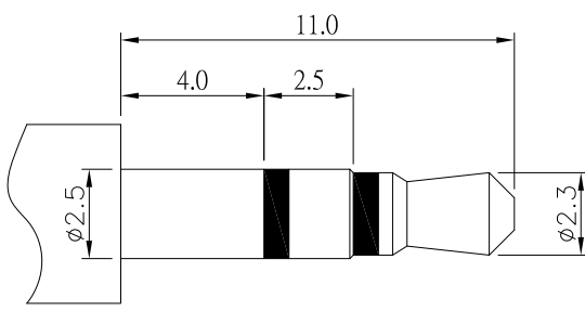
φ2.50mm 3 POLE PLUG
