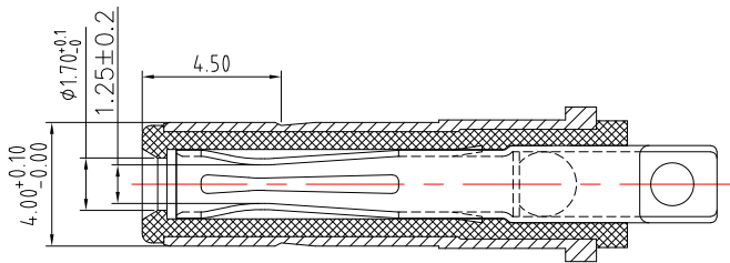
MATING PLUG
