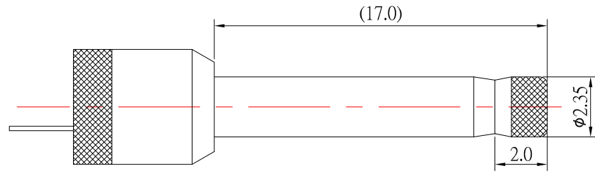
RECOMMENDED PLUG
