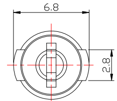
RECOMMENDED PLUG
