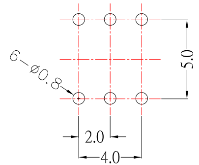
P.C.B MOUNTING PATTERN
