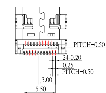
USB TYPE-C PIN ASSIGNMENTS
