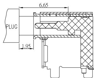
mating drawing
