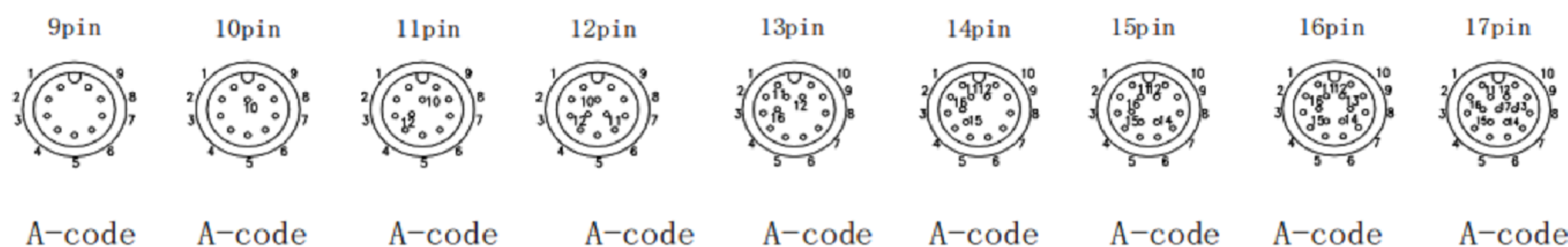
Pin assignment front view/针位分布前视图
