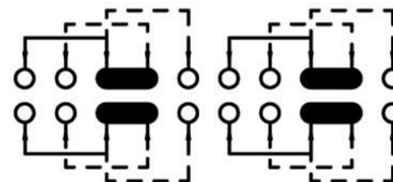
SCHEMATIC (NON-SHORTING)
