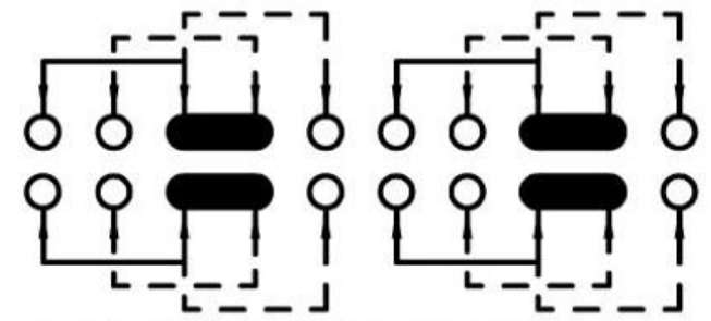
SCHEMATIC (NON-SHORTING)
