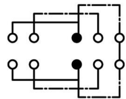
SCHEMATIC (NON-SHORTING)
