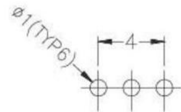
P.C.B LAYOUT MOUNTING PATTERN
