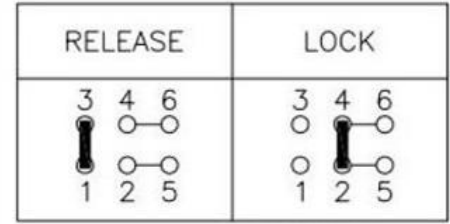
SCHEMATIC (NON-SHORTING)
