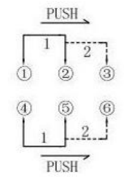
SCHEMATIC (NON-SHORTING)
