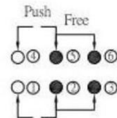
SCHEMATIC (NON-SHORTING)
