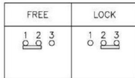
SCHEMATIC (NON-SHORTING)
