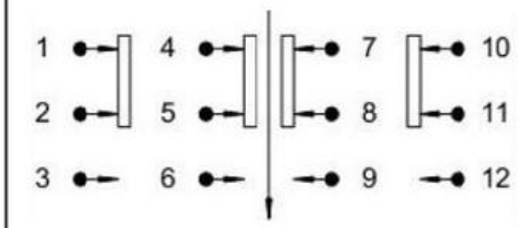
SCHEMATIC (NON-SHORTING)
