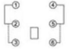
SCHEMATIC (NON-SHORTING)
