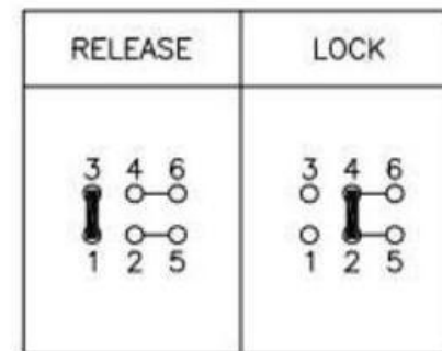
SCHEMATIC (NON-SHORTING)
