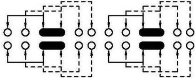
SCHEMATIC (NON-SHORTING)
