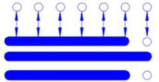
SCHEMATIC (NON-SHORTING)
