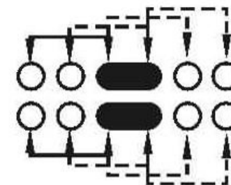
SCHEMATIC (NON-SHORTING)
