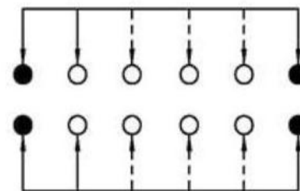
SCHEMATIC (NON-SHORTING)
