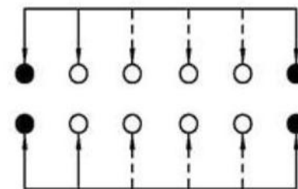
SCHEMATIC (NON-SHORTING)
