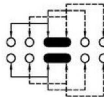
SCHEMATIC (NON-SHORTING)
