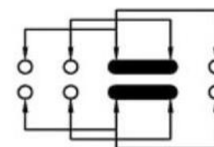
SCHEMATIC (NON-SHORTING)
