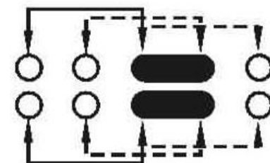
SCHEMATIC (NON-SHORTING)
