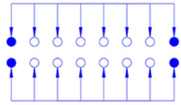
SCHEMATIC (NON-SHORTING)
