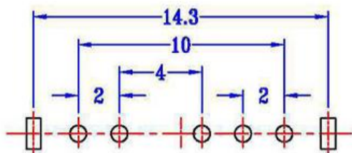
P.C.B LAYOUT BOTTOM VIEW
