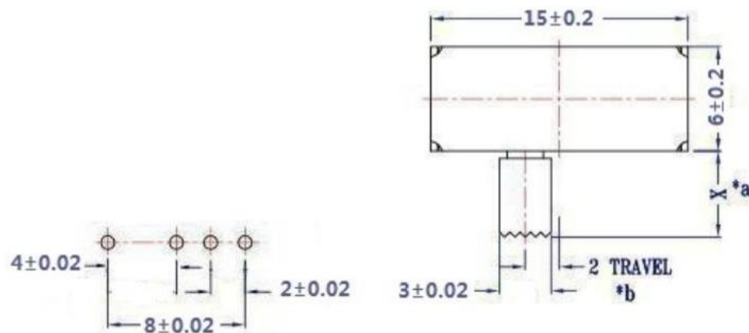
P.C.B LAYOUT BOTTOM VIEW
