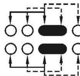
SCHEMATIC (NON-SHORTING)
