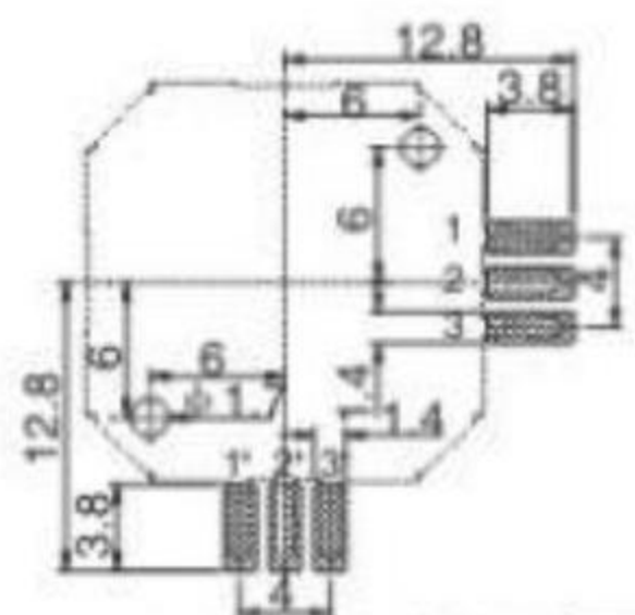
Recommended PAD LAYOUT ±0.05 TOP VIEW
