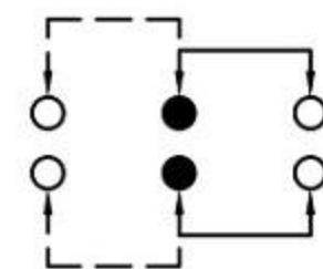
SCHEMATIC (NON-SHORTING)
