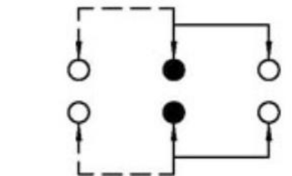
SCHEMATIC (NON-SHORTING)
