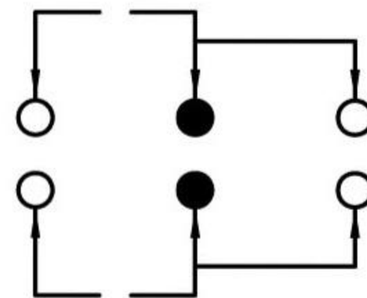
SCHEMATIC (NON-SHORTING)
