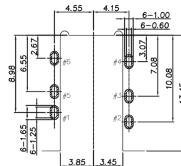
RECOMMENDED P.C.B LAYOUT TOP VIEW (TOLRANCE: \pm 0.05 )
