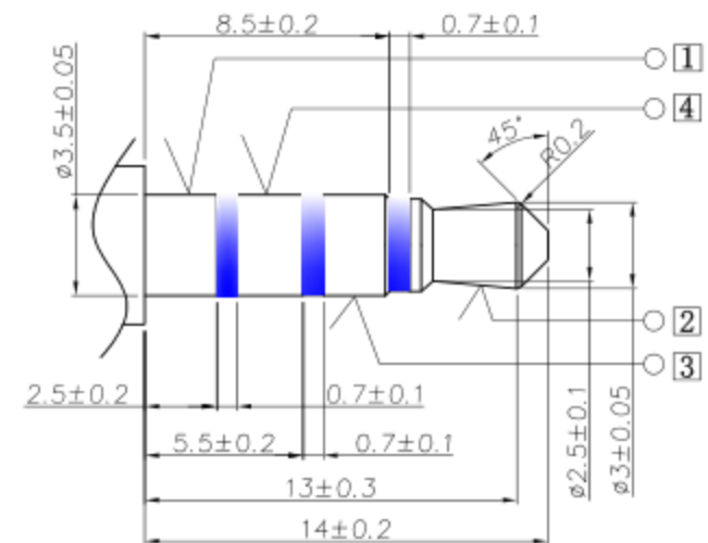
Matching Plug
