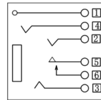
Circuit Diagram
