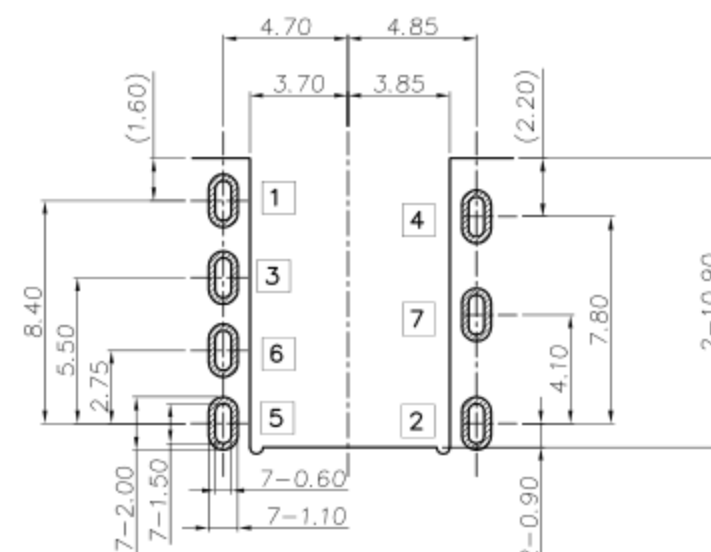
RECOMMENDED P.C.B LAYOUT (t=1.0mm) TOP VIEW (TOLRANCE: ±0.05)
