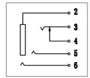
SCHEMATIC
