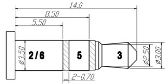
3.5 PLUG SPEC
